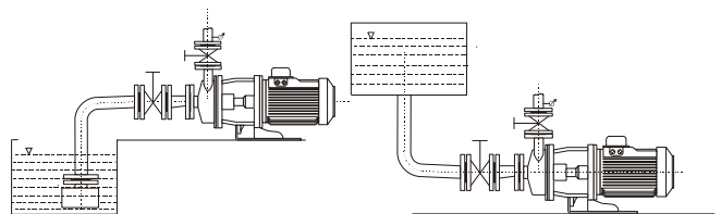
Fig. 2 Pipe connection
