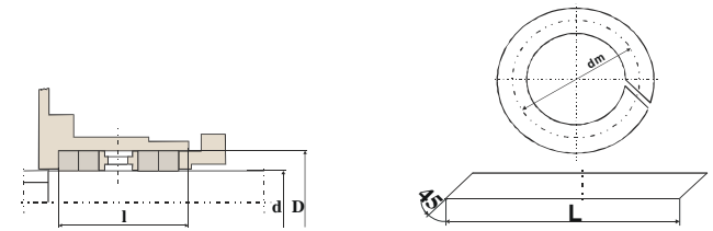
Fig.3 Packing gland
